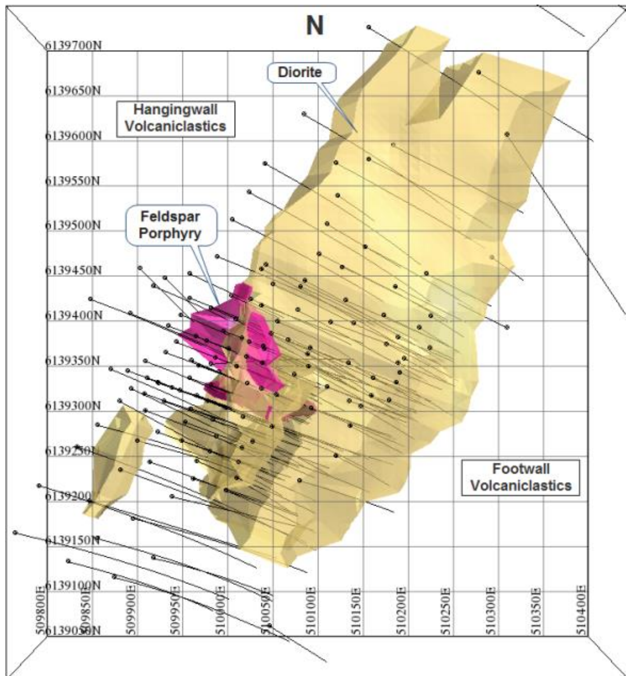
Figure 6.14: Lithological Model.
